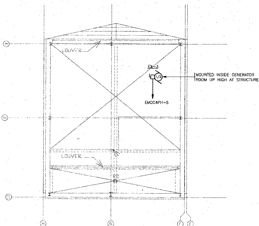
2 PART PLAN: EMERGENCY GENERATOR ROOM UPPER LEVEL
