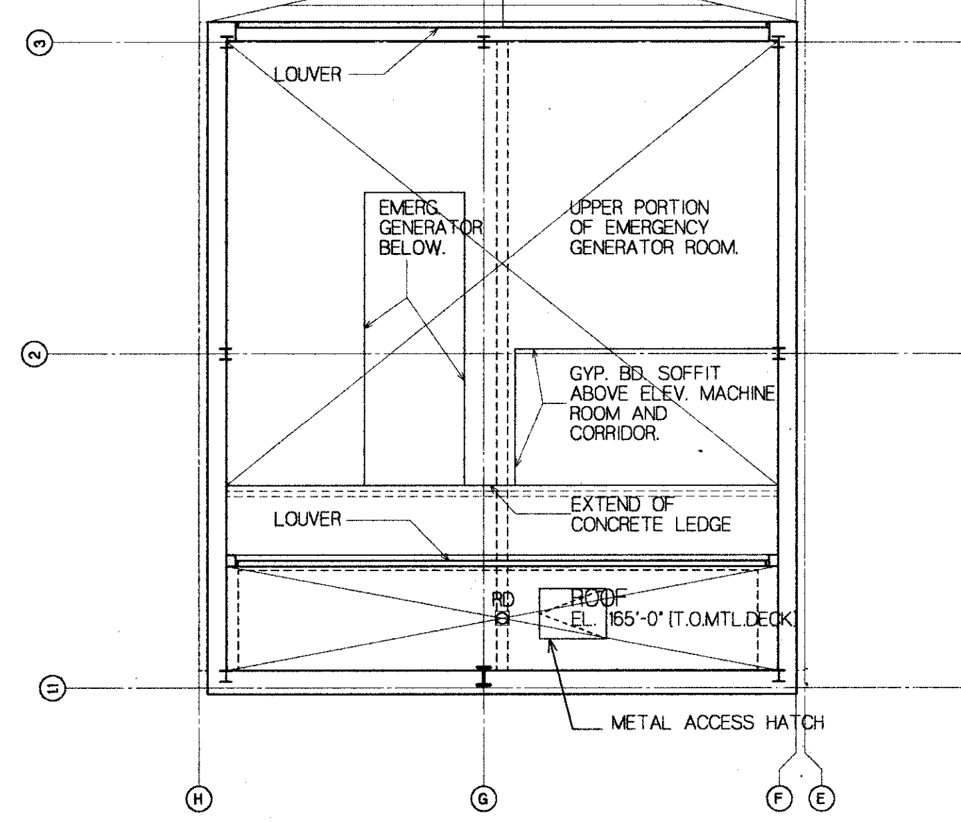
2 PART. PLAN: EMERGENCY GENERATOR ROOM UPPER LEVEL
