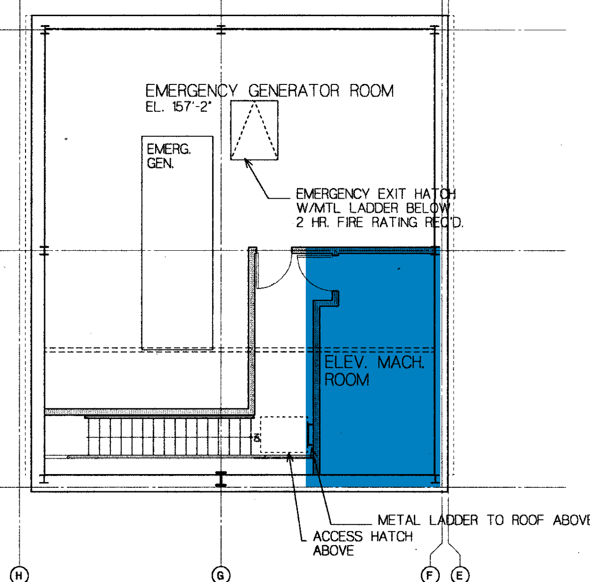
1 PART. PLAN: EMERGENCY GENERATOR ROOM
