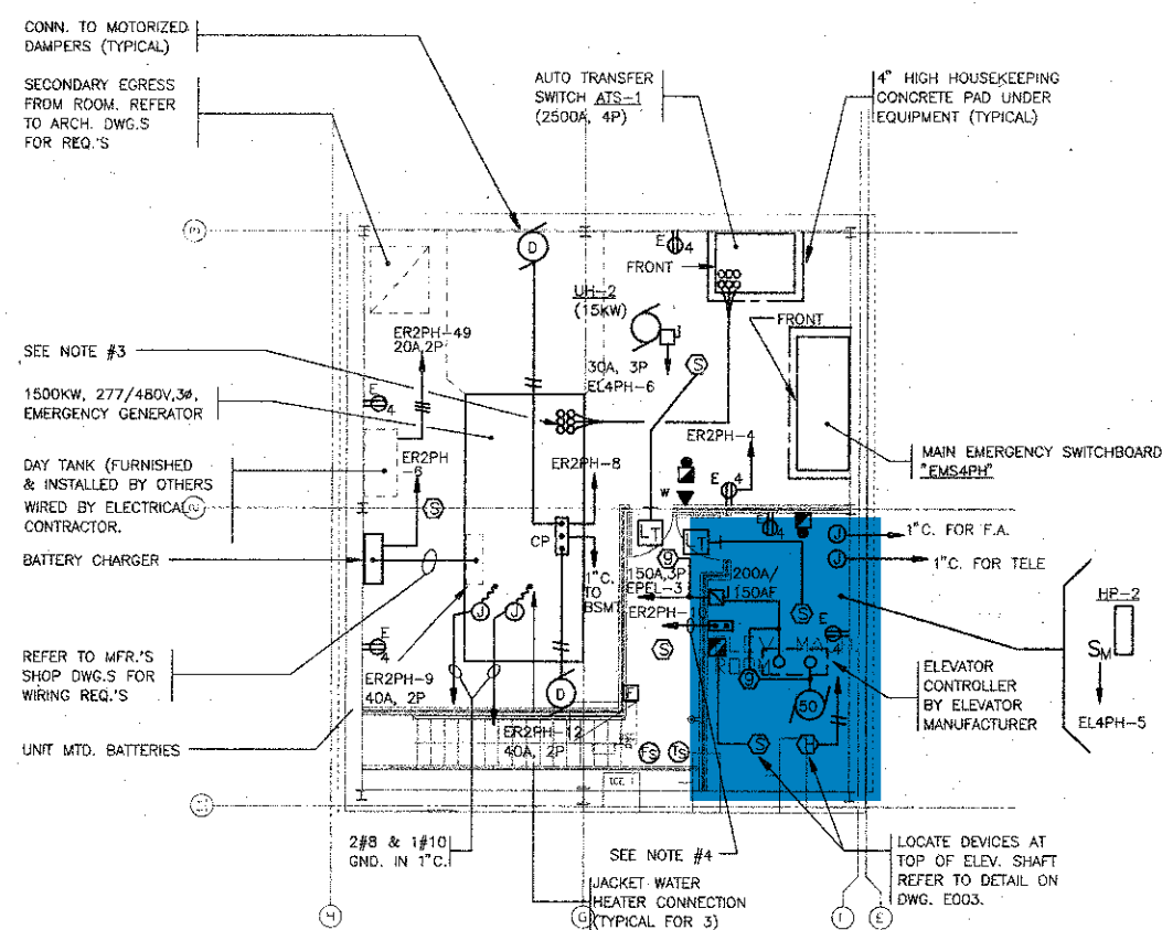
3 PART PLAN: EMERGENCY GENERATOR ROOM POWER PLAN
